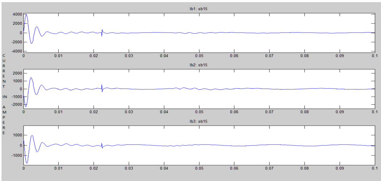
Figure 15: Current Waveform of Bus 1 without Series Compensator
