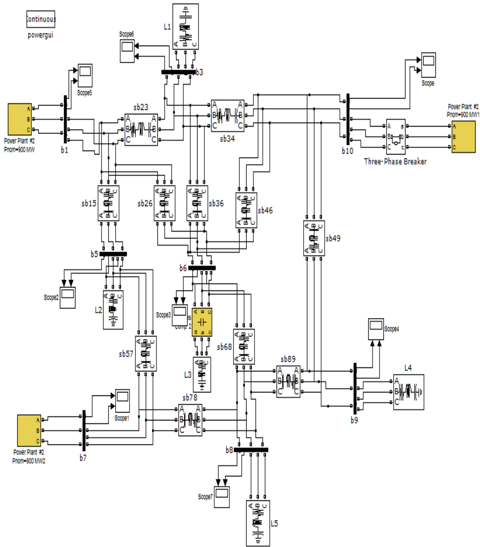
Figure 8: Simulation model of 11 bus system with series compensator
