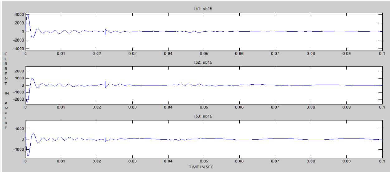
Figure 16: Current Waveform of Bus 1 with Series Compensator
