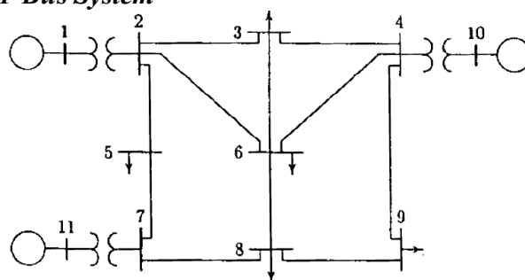
Figure 6: Single Line diagram of 11-bus power system
