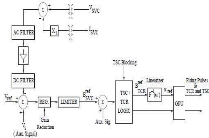
Figure 4: SVC Controller
