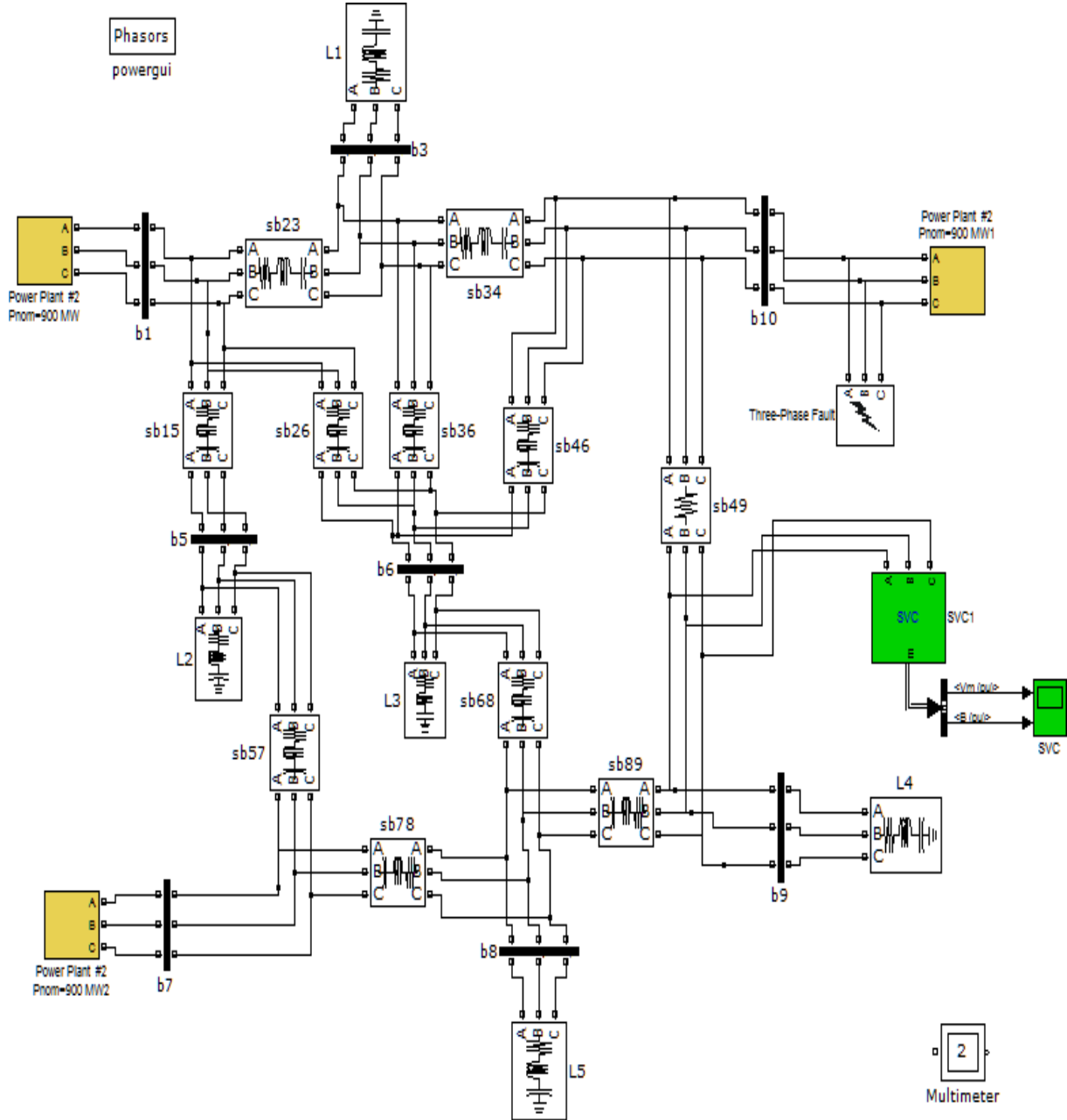
Figure 7: Simulation model of 11-bus system with SVC
