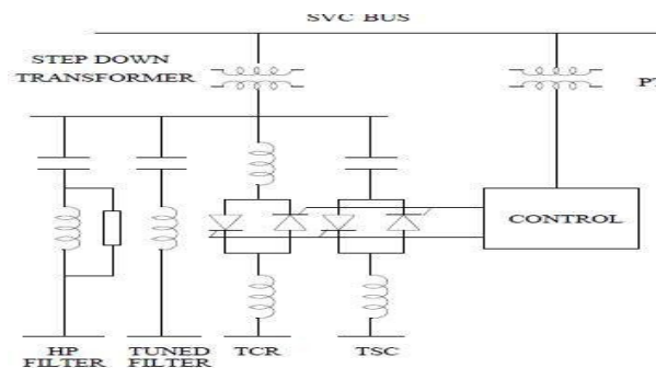
Figure 3: A Typical SVC (TSC-TCR) Configuration
