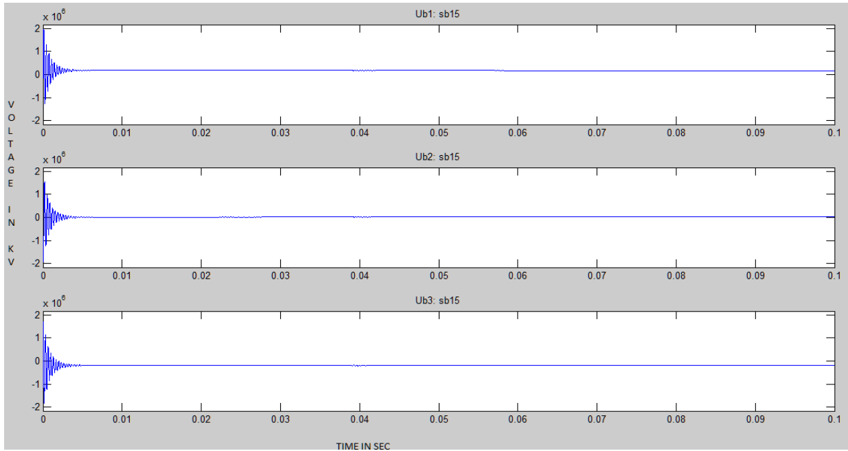
Figure 10: Voltage Waveform of Bus 10 with SVC
