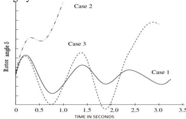
Figure 2: Rotor angle response to a transient disturbance.
