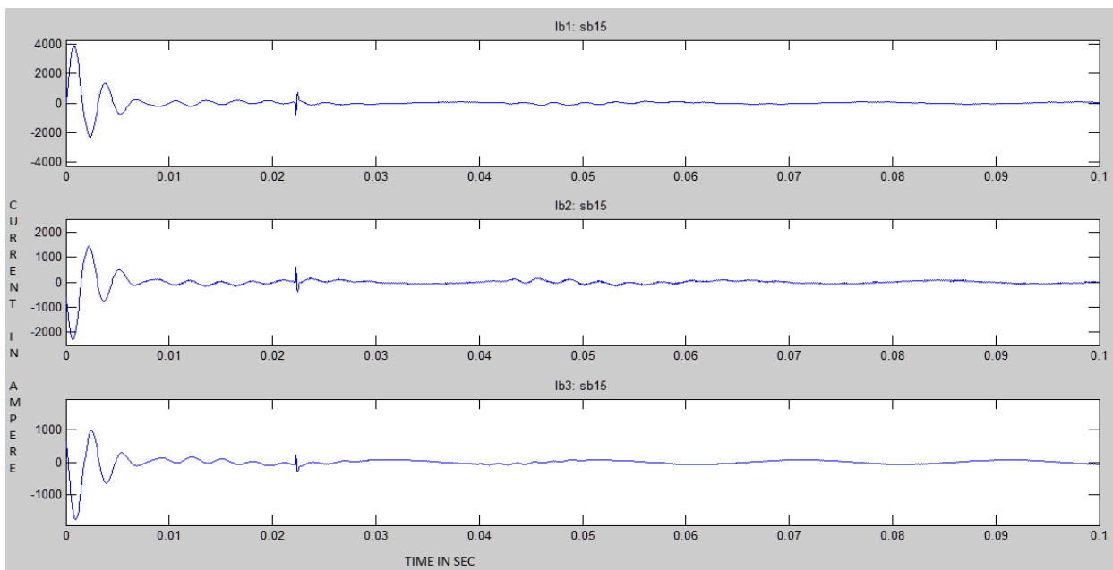
Figure 11: Current Waveform of Bus 10 without SVC
