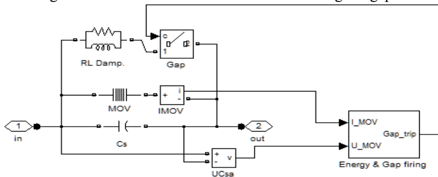
Figure5: Series Compensation of Subsystem
