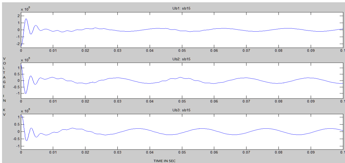
Figure 13: Voltage Waveform of Bus 1 without Compensator
